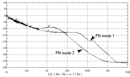
Phase noise modes 1 and 2 at fc = 900 MHz
